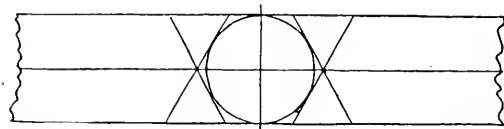
FIG. 552. LAYING OUT JOINT FOR SIX-ARM PATTERN.
